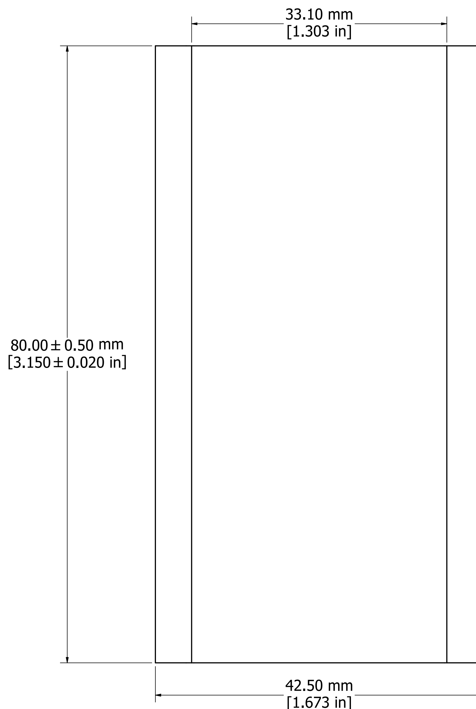
EXTRUSION PROFILE
