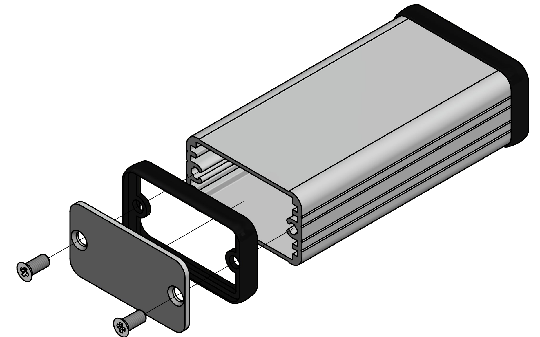
EXPLODED ASSEMBLY VIEW
