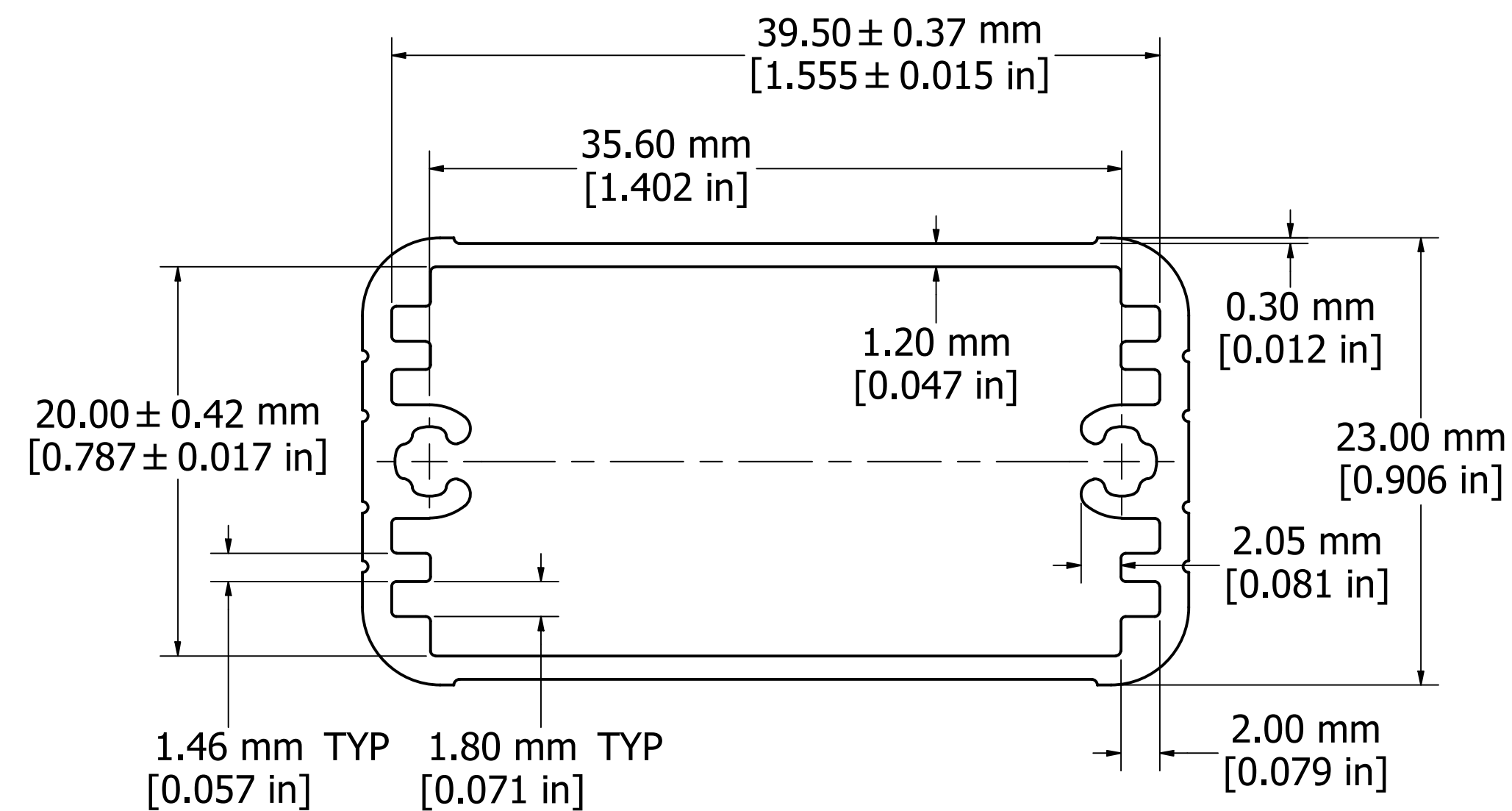
EXTRUSION PROFILE
