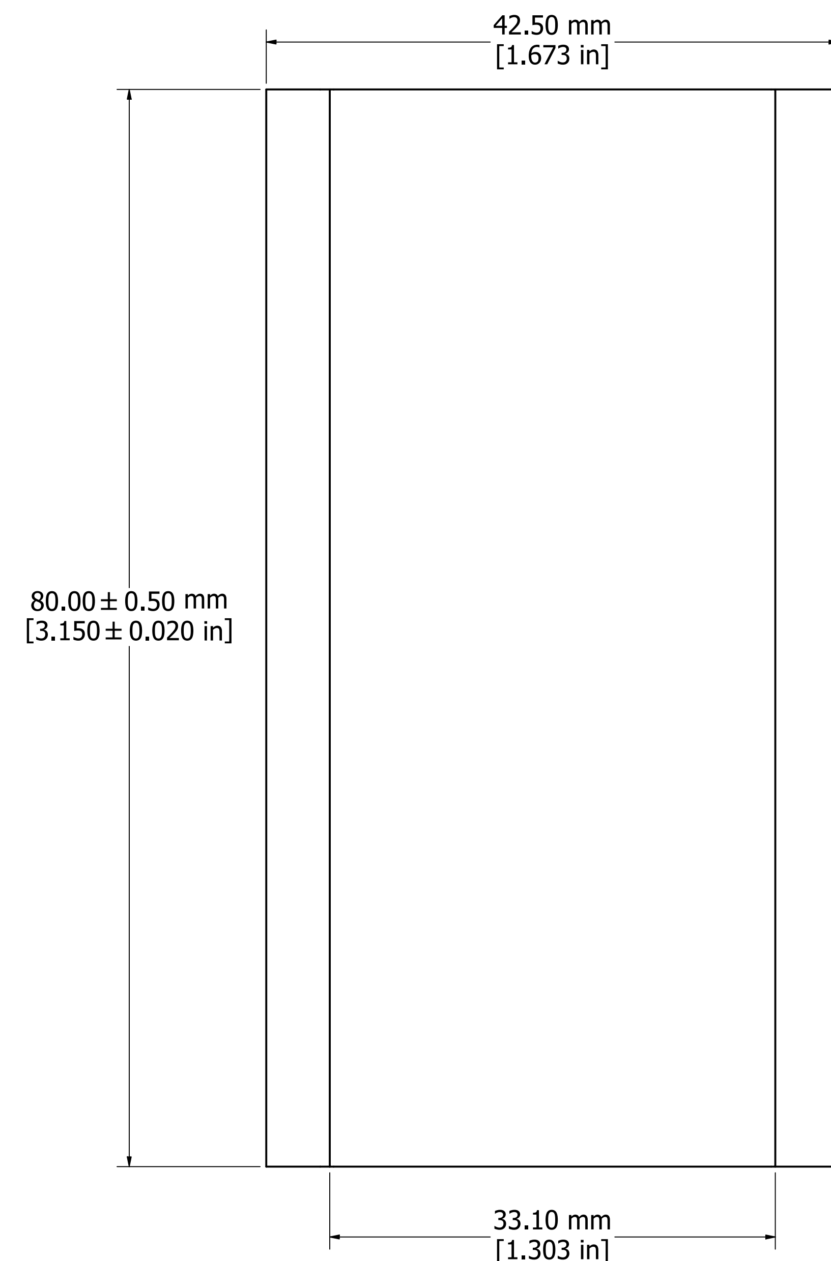
EXTRUSION PROFILE
