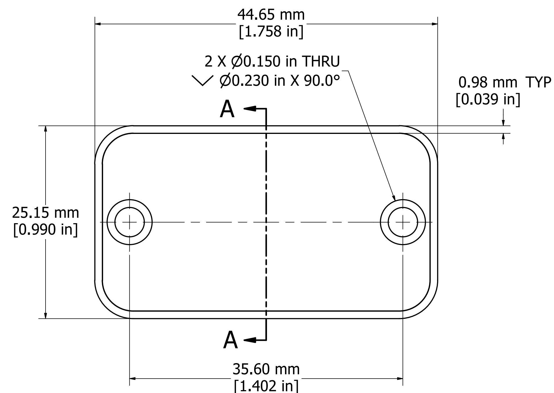
CLOSED BEZEL
