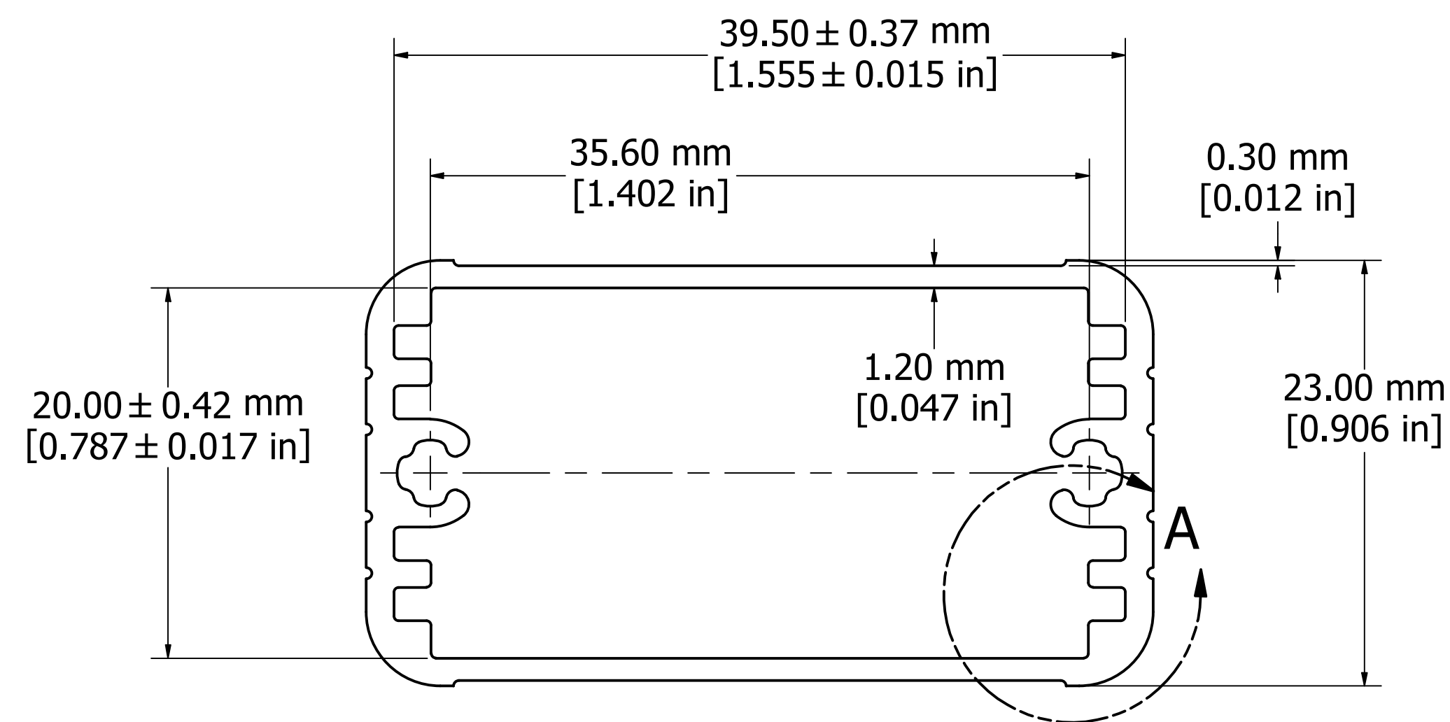
EXTRUSION PROFILE
