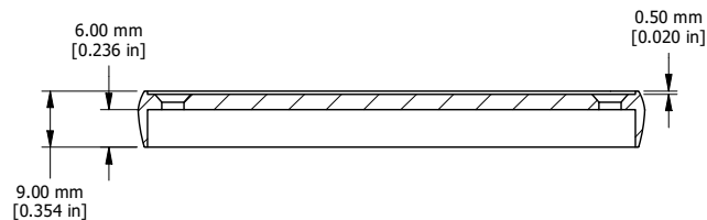
CLOSED BEZEL
