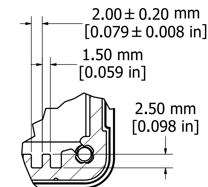
DETAIL A
