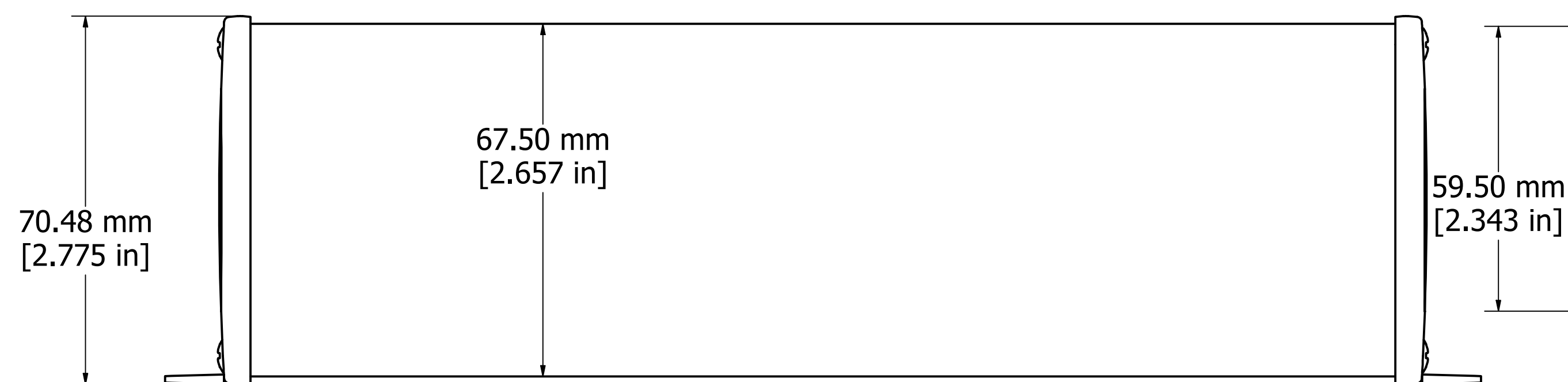
ASSEMBLY - VIEW FROM TOP
