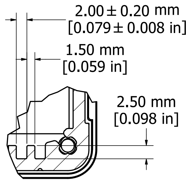
DETAIL A
