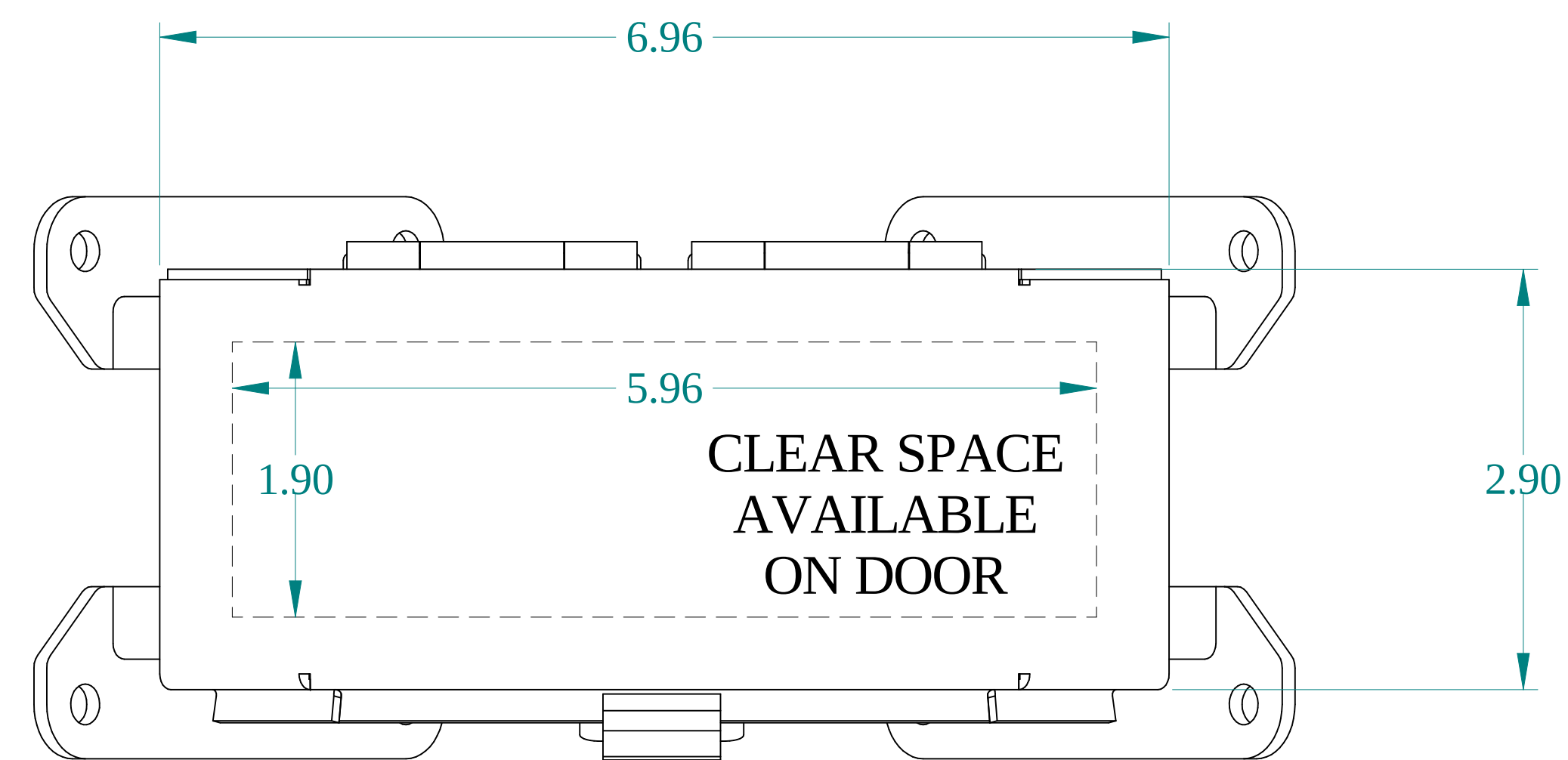
TOP VIEW
