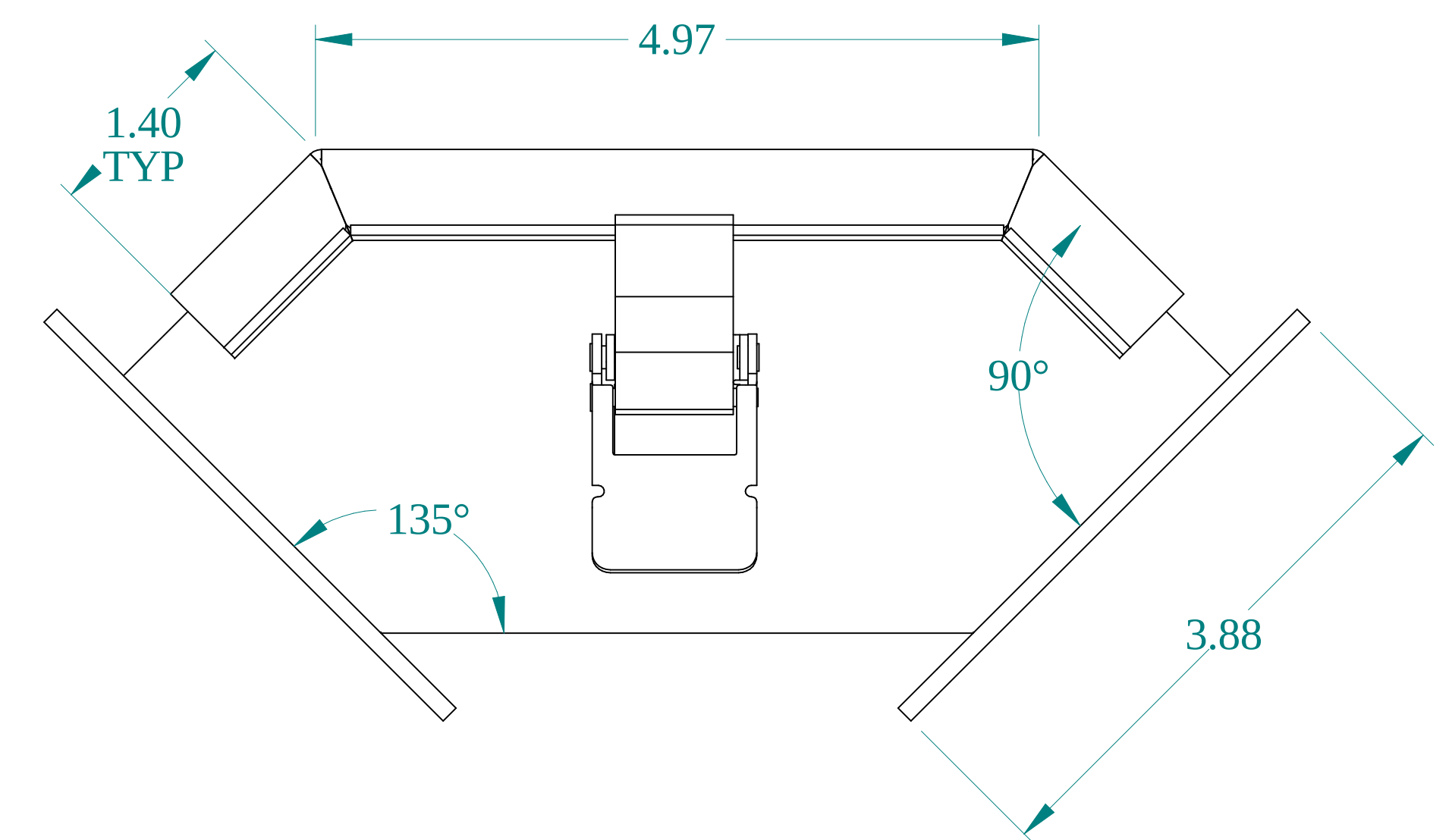
BACK VIEW
