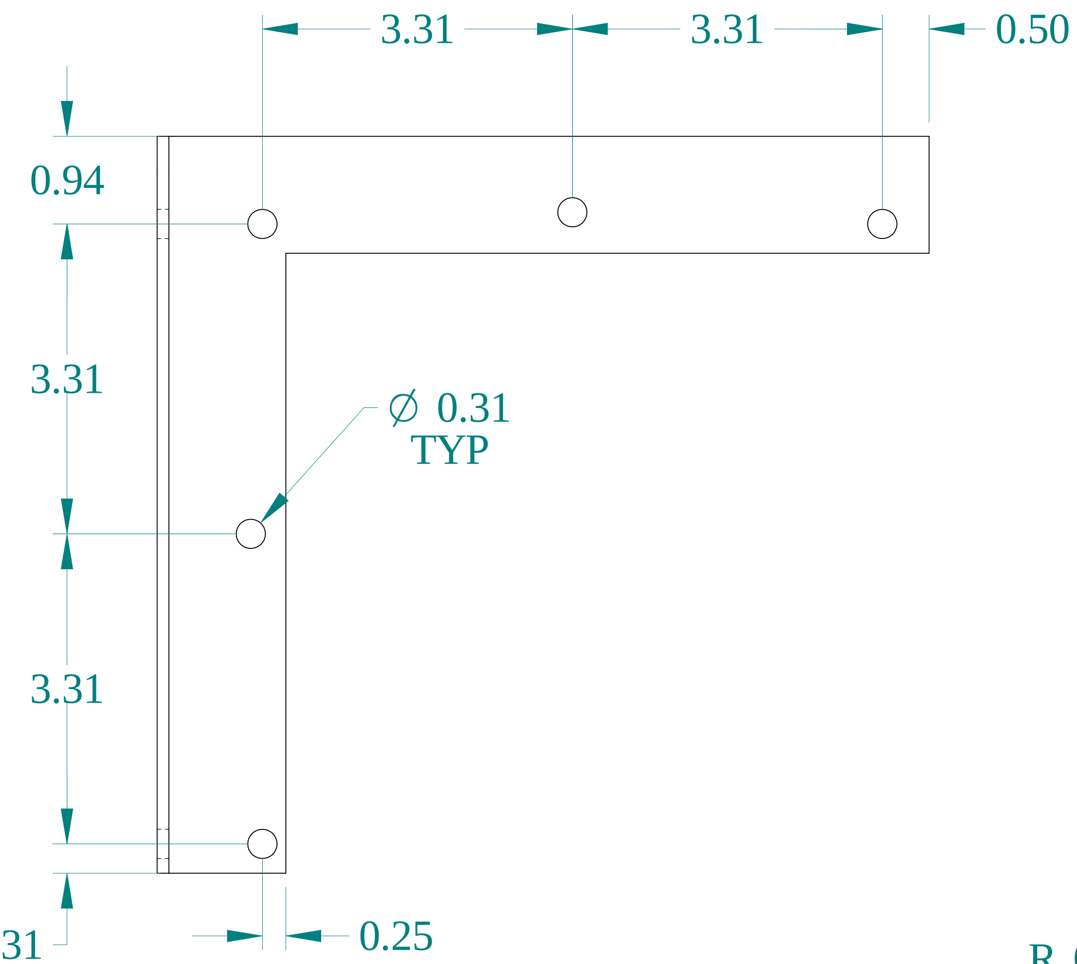
FRONT VIEW
