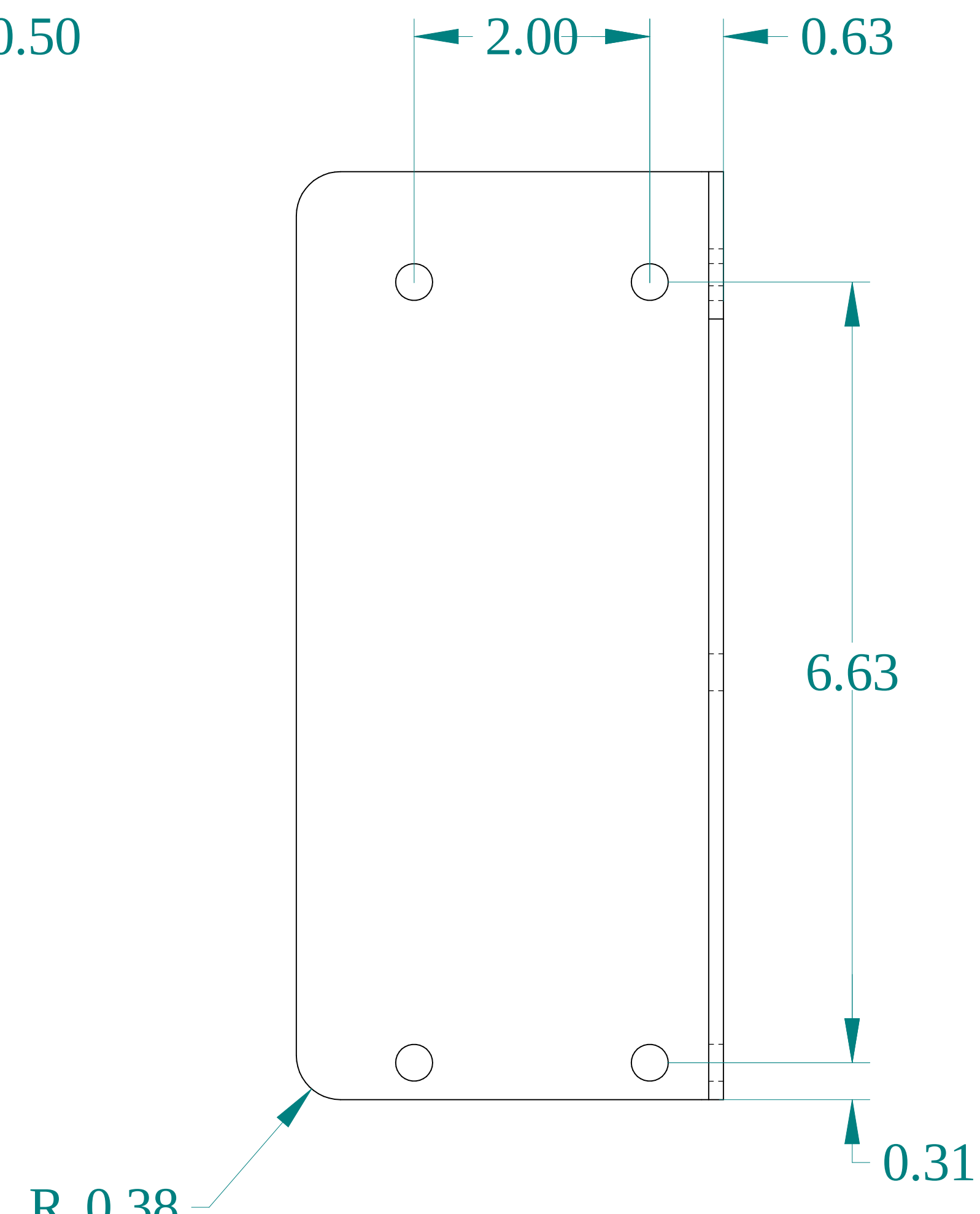
SIDE VIEW
