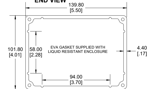
SECTION A-A END VIEW
