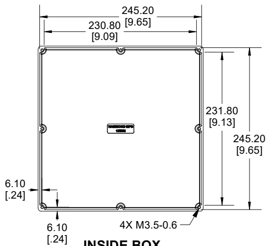
INSIDE BOX
