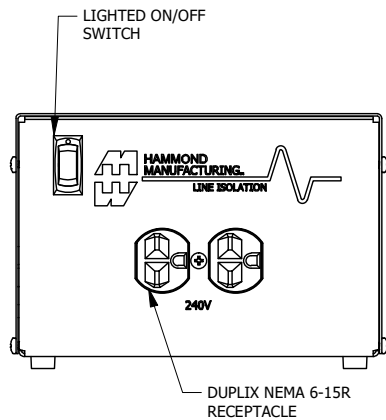
ASSEMBLY - FRONT VIEW
