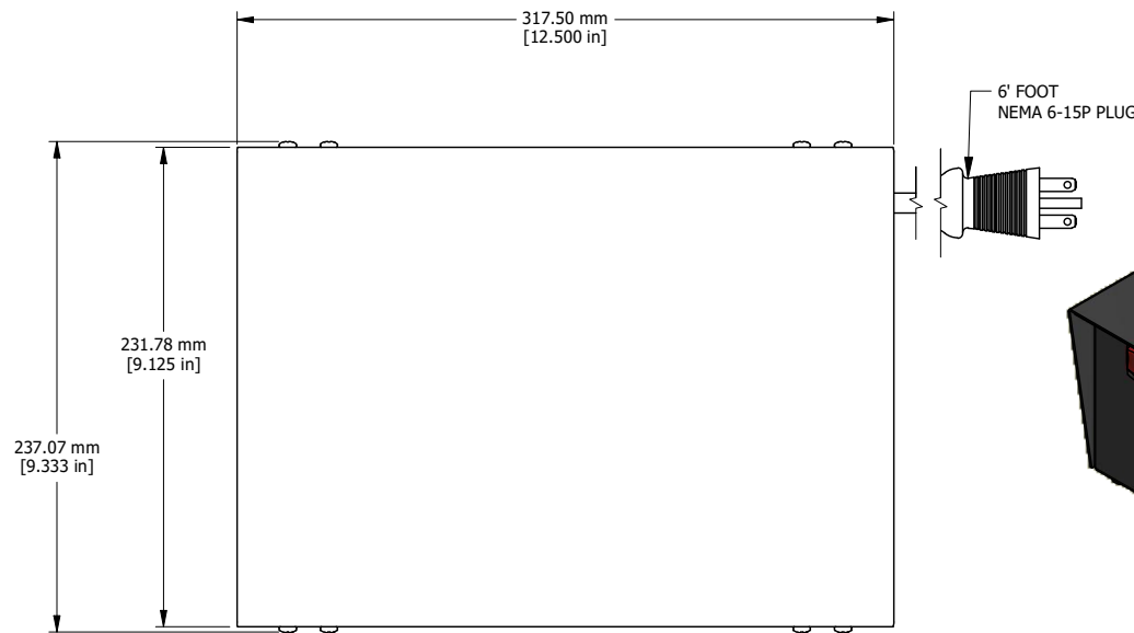
ASSEMBLY - TOP VIEW
