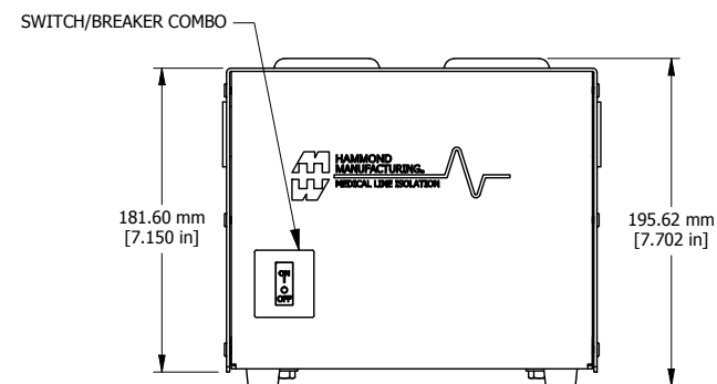
ASSEMBLY - VIEW FROM FRONT
