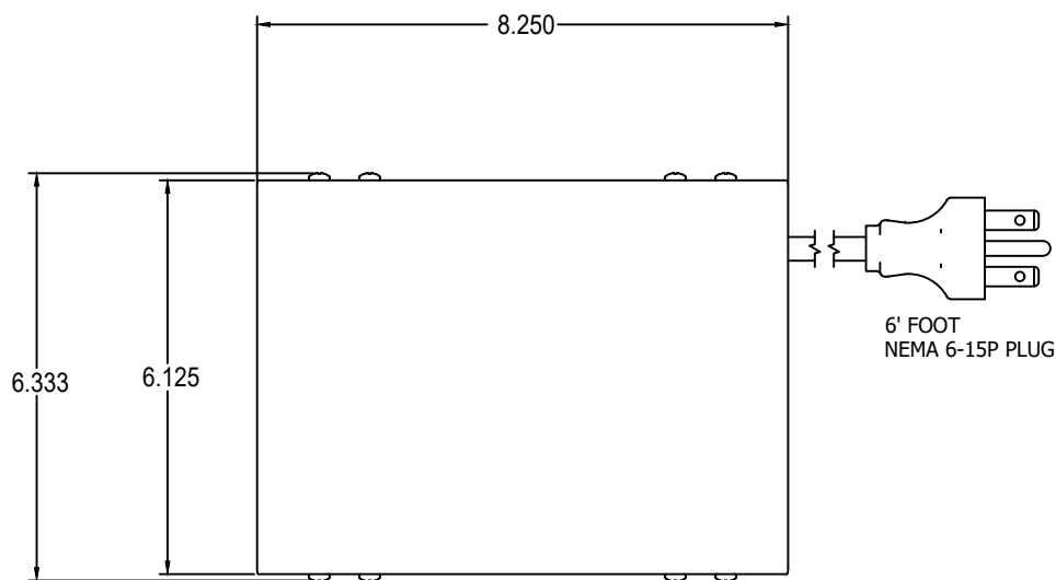
ASSEMBLY - TOP VIEW
