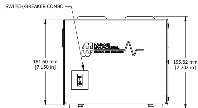
ASSEMBLY - VIEW FROM FRONT
