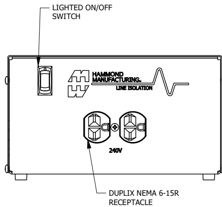
ASSEMBLY - FRONT VIEW
