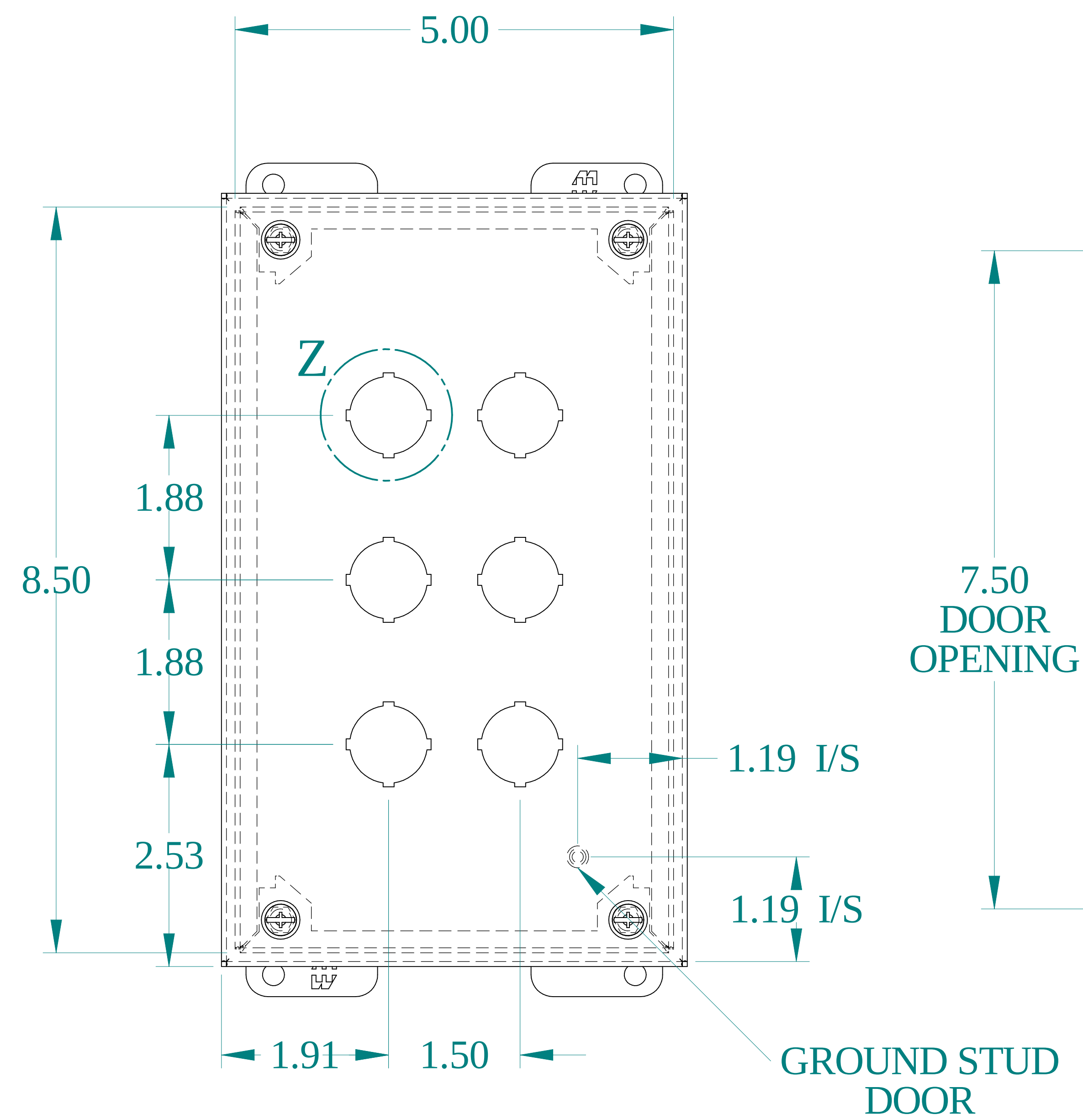
TOP VIEW
