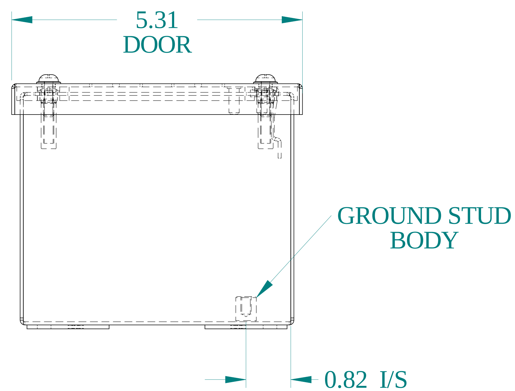
BOTTOM VIEW
