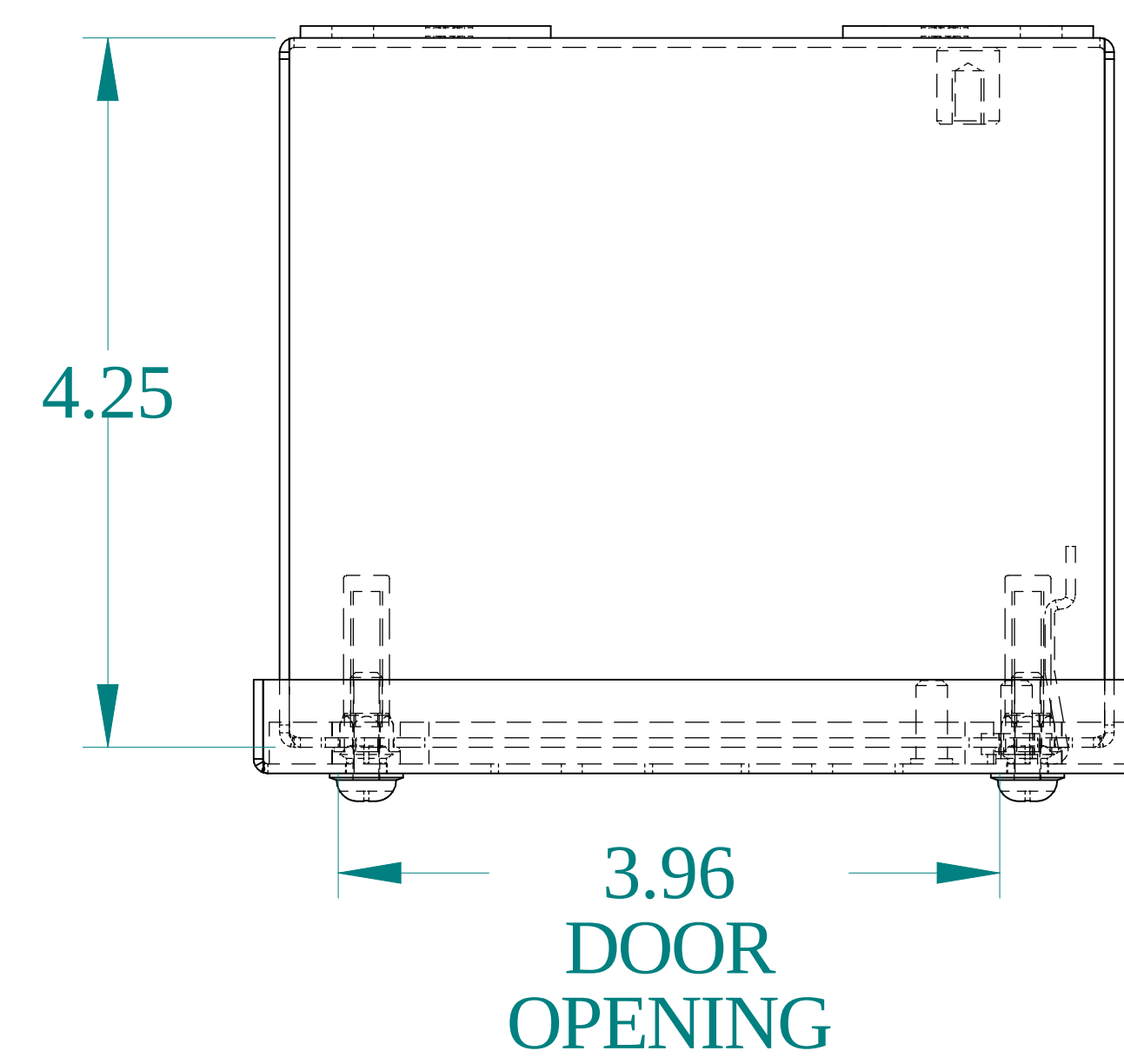
TOP VIEW
