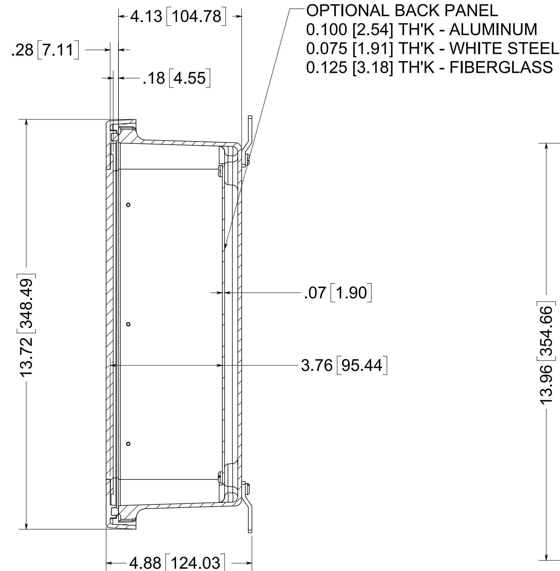
SECTION B-B
