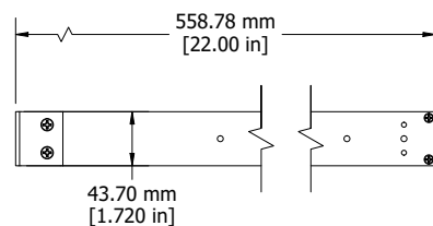
ASSEMBLY - FRONT VIEW
