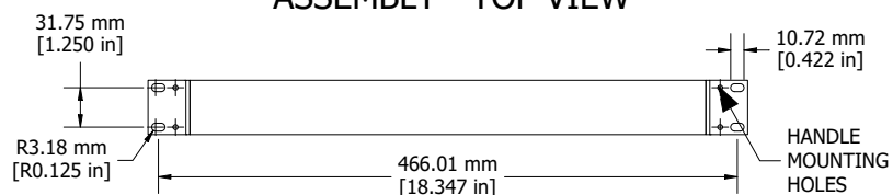
ASSEMBLY - TOP VIEW
