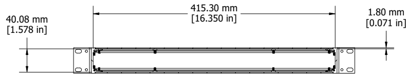
SECTION B-B
