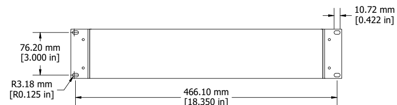
ASSEMBLY - FRONT VIEW
