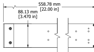
ASSEMBLY - SIDE VIEW
