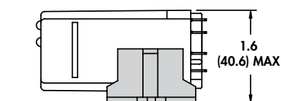
HORIZONTAL MOUNT (All Mating Relays)
