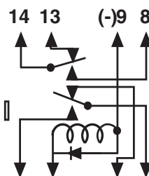
Figure S DPDT With diode
