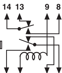
Figure R DPDT Without diode
