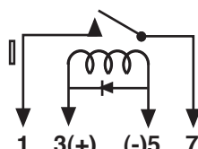
Figure C SPST-NO With diode
