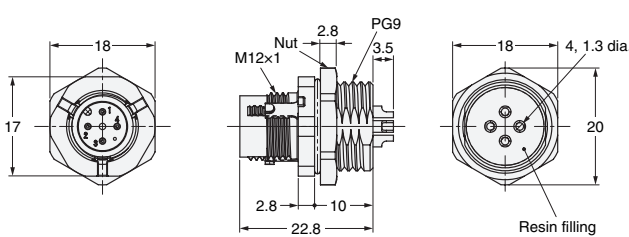
XS5M-D427-4 Front-locking Plug with Solder Cup Pins
