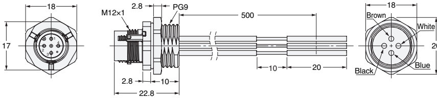
XS5M-D427-5 Front-locking Plug Connected to Wires
