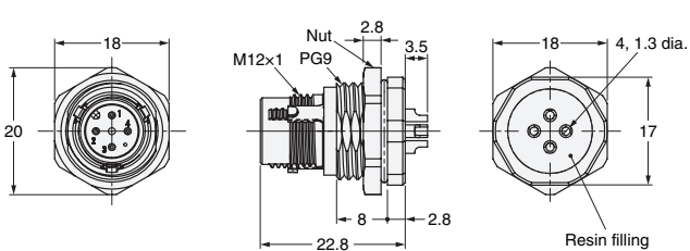
XS5M-D427-4 Front-locking Plug with Solder Cup Pins
