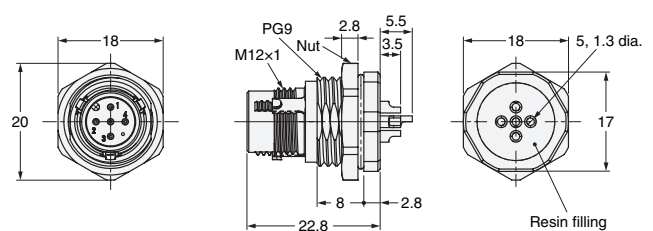
XS5M-D527-4 Front-locking Plug with Solder Cup Pins
