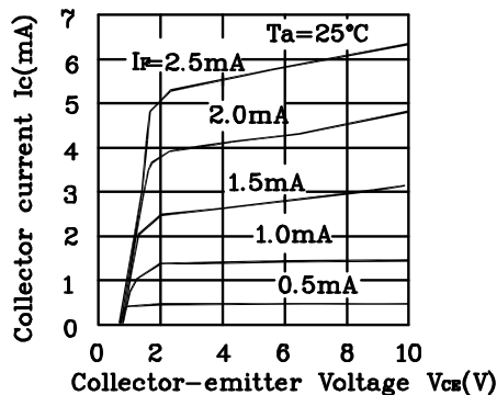
Fig.3 COLLECTOR CURRENT Vs. COLLECTOR-EMITTER VOLTAGE
