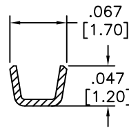
C-C SEC.
