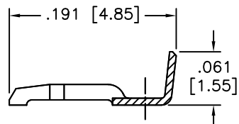
B-B SEC.
