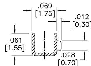
D-D SEC.
