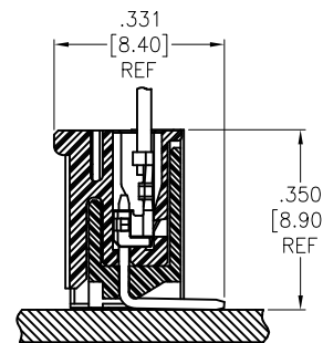
ASSEMBLY VIEW
