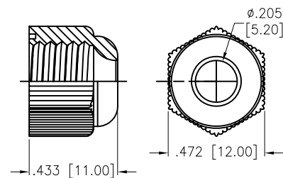
Ⓔ Sealing Nut
