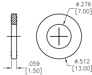
Ⓑ Washer
