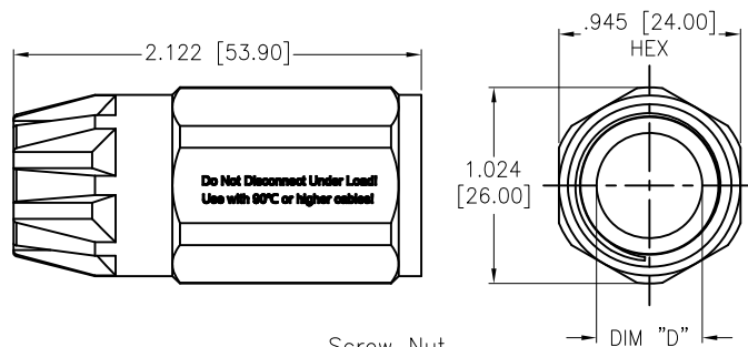
Screw Nut
