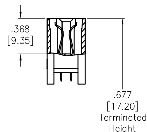
CONTACT DETAIL
