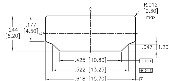
REFERENCE PANEL CUT OUT DIMENSION
