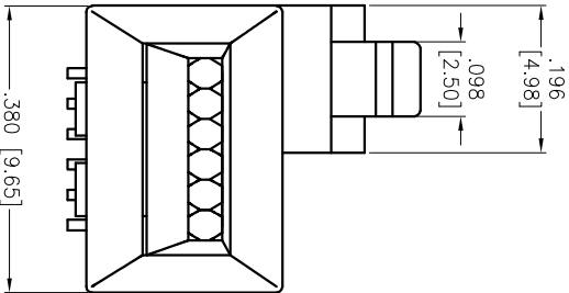
BACK VIEW
