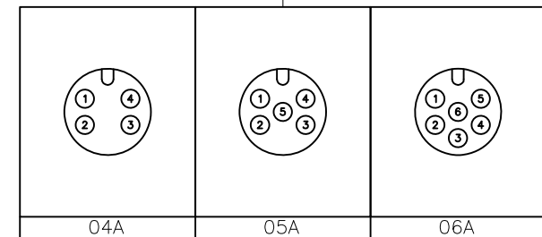
PIN ASSIGNMENT FRONT VIEW
