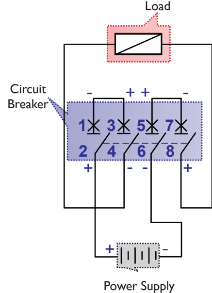
Figure 4: Four Pole, Double Break. Isolates Load (400 Vdc)
