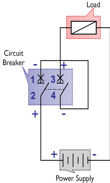
Figure 2: Double Pole, Single Break (600 Vdc)
