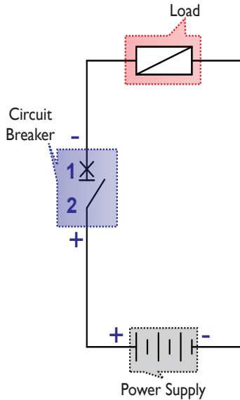
Figure 1: Single Pole, Single Break (300 Vdc)
