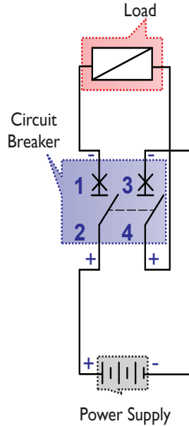
Figure 3: Double Pole, Double Break. Isolates Load (300 Vdc, 400 Vdc, 600 Vdc)
