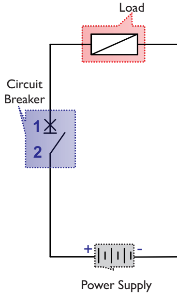
Figure 1: Single Pole, Single Break (150 Vdc)
