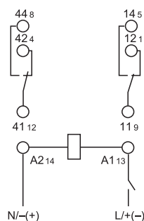
Wiring diagram (without control signal)
