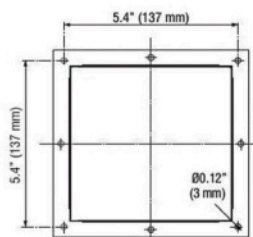
Drilling template for mounting frame
