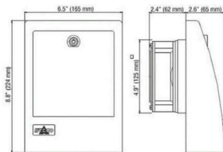
Outdoor Filter Fan
