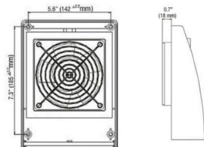
View from rear Outdoor Exhaust Filter
