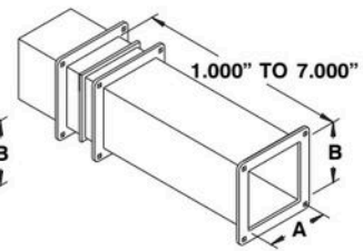
TELESCOPE FITTINGS
