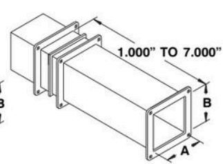
TELESCOPE FITTINGS
