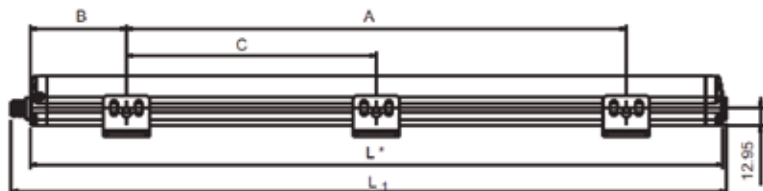
Installation with anti-vibration supports
