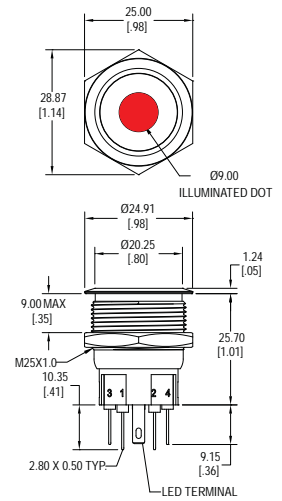
C Non-Latching
