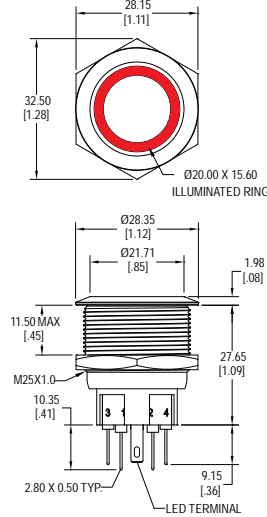
B Non-Latching
