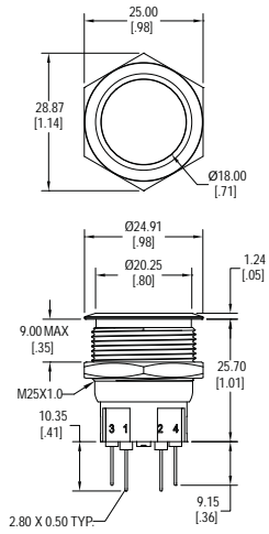
A Non-Latching
