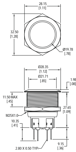
A Non-Latching
