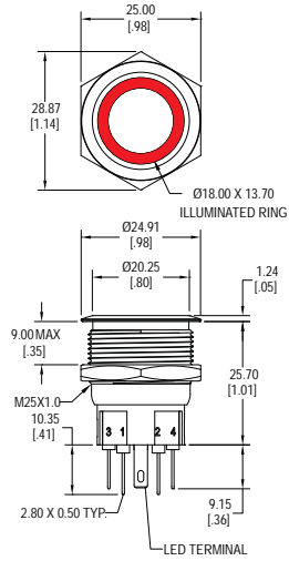
B Non-Latching
