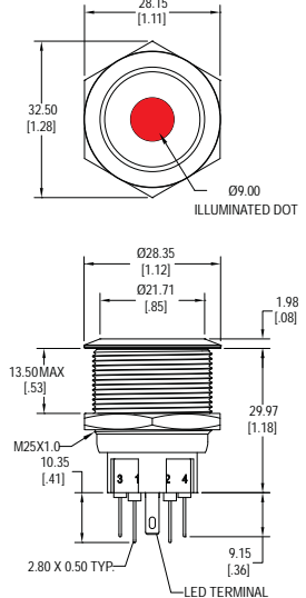
C Latching
