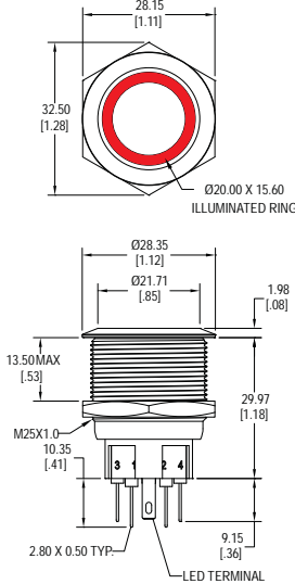
B Latching
