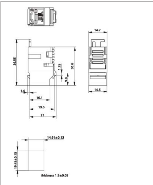
PC Board Layout - Component Side
