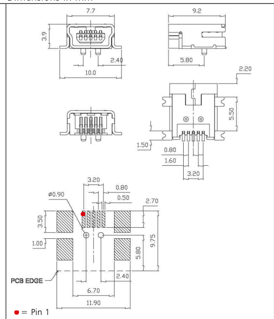
PC Board Layout - Top View
