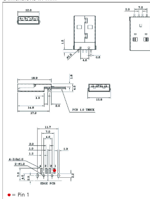
PC Board Layout - Component Side
